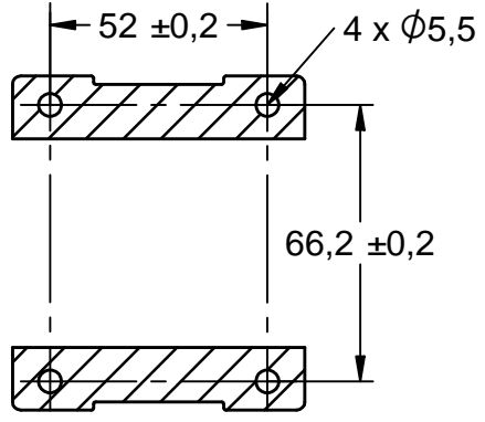
Fastening plate A-A
