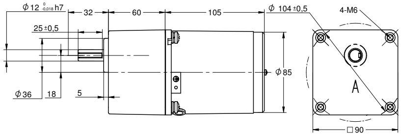
DRAWING (mm)
